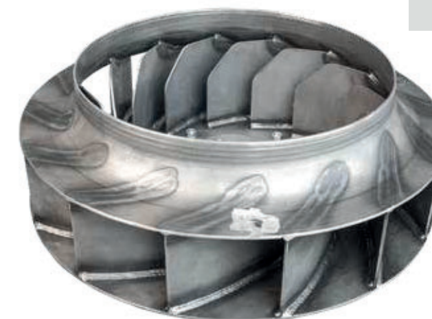
heavy process air fan wheel made of N-A-XTRA® with balancing point
